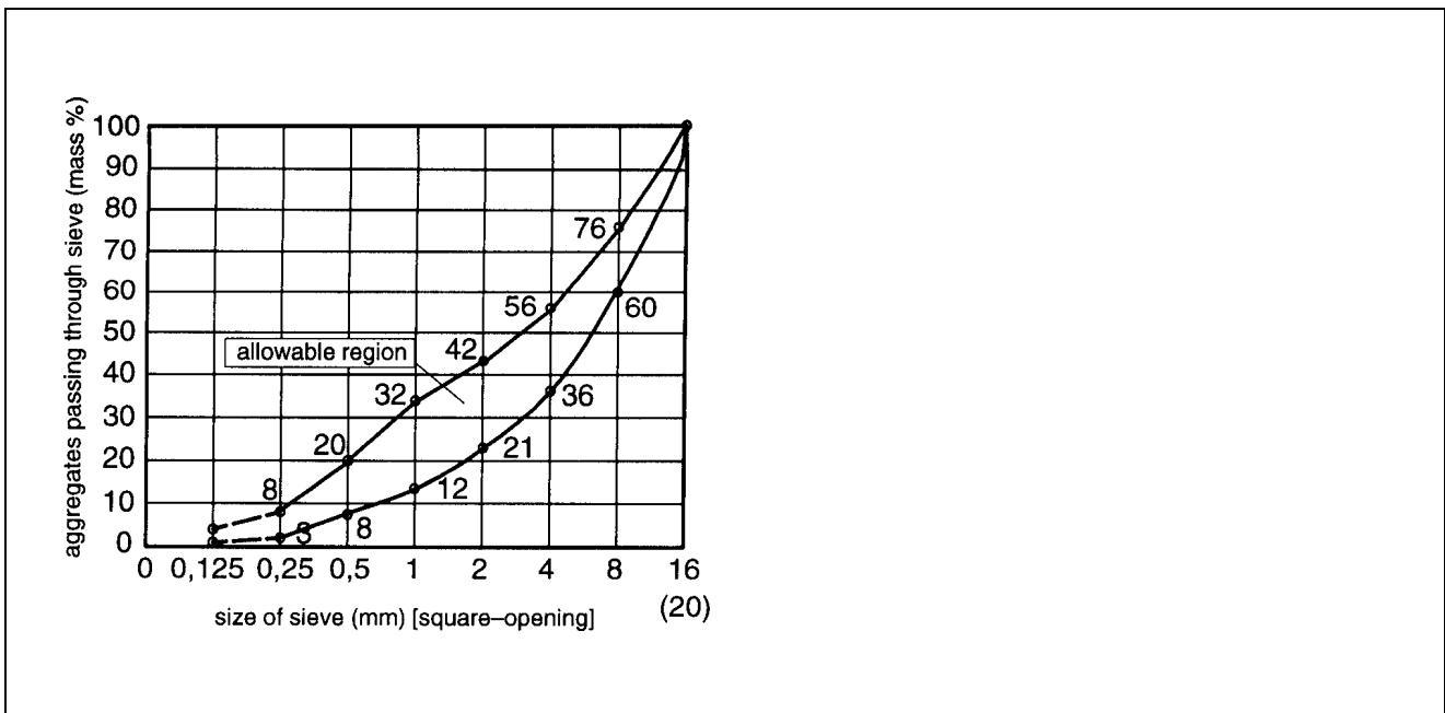
Figure C.2.1 Admissible region for the grading curve
