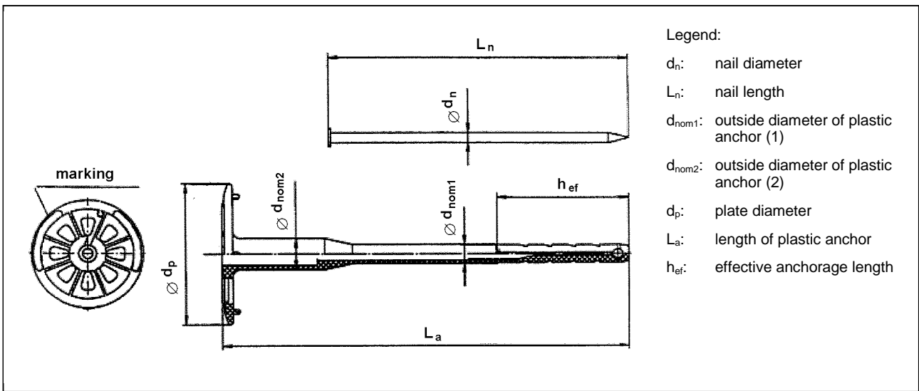
Figure 2.1b: Components of plastic anchor
