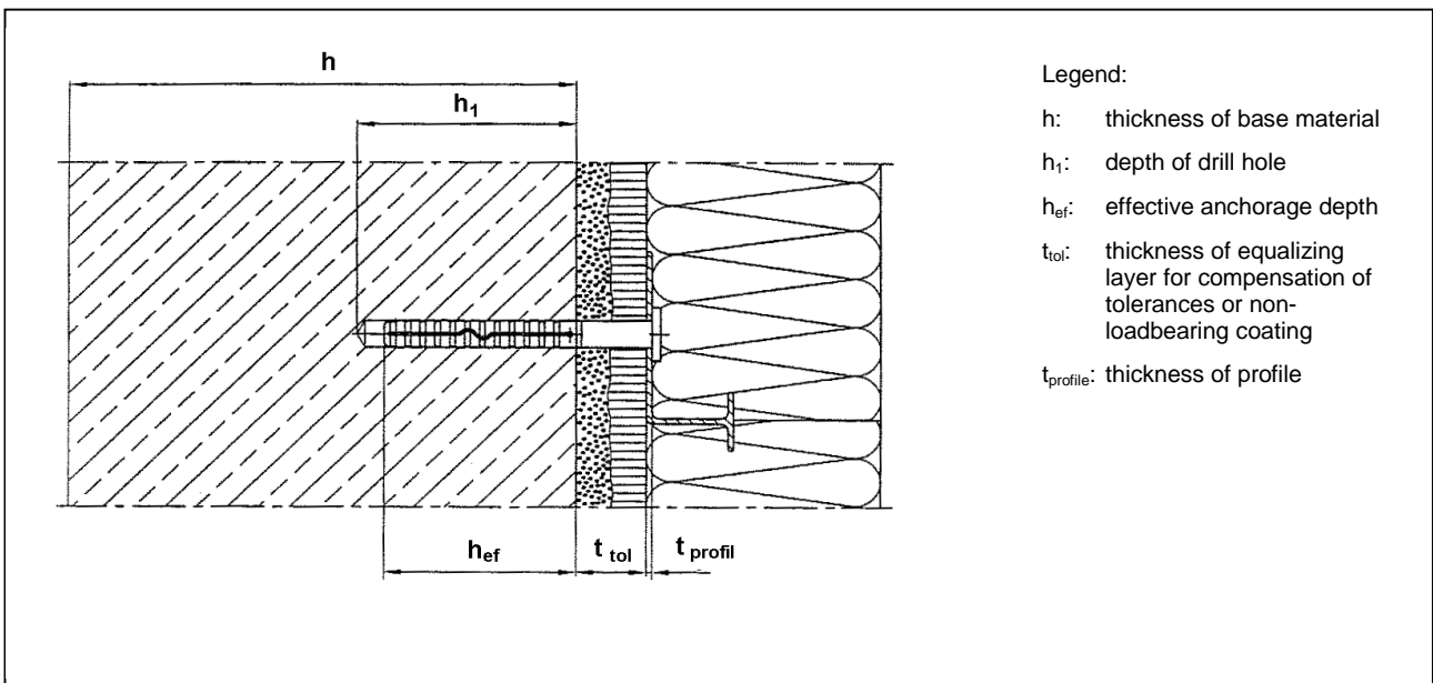
Figure 2.2: Plastic anchors for profiles for ETICS
